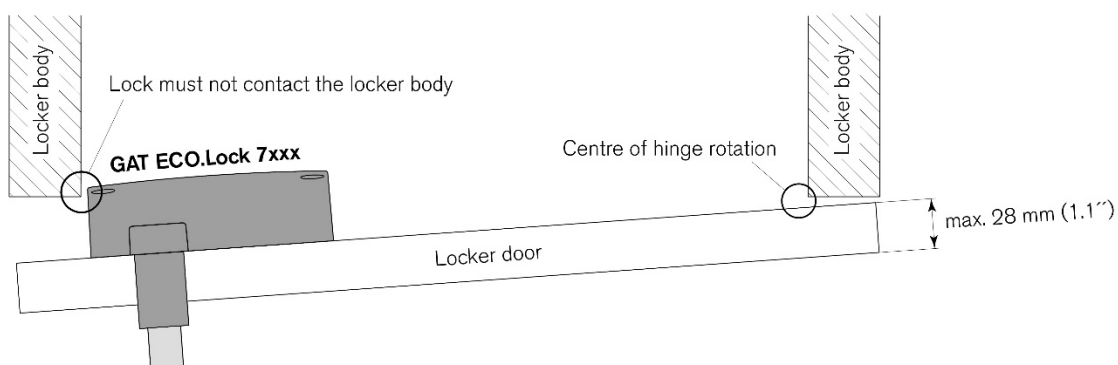
Fig. 3.2 – Width and thickness of the locker door
