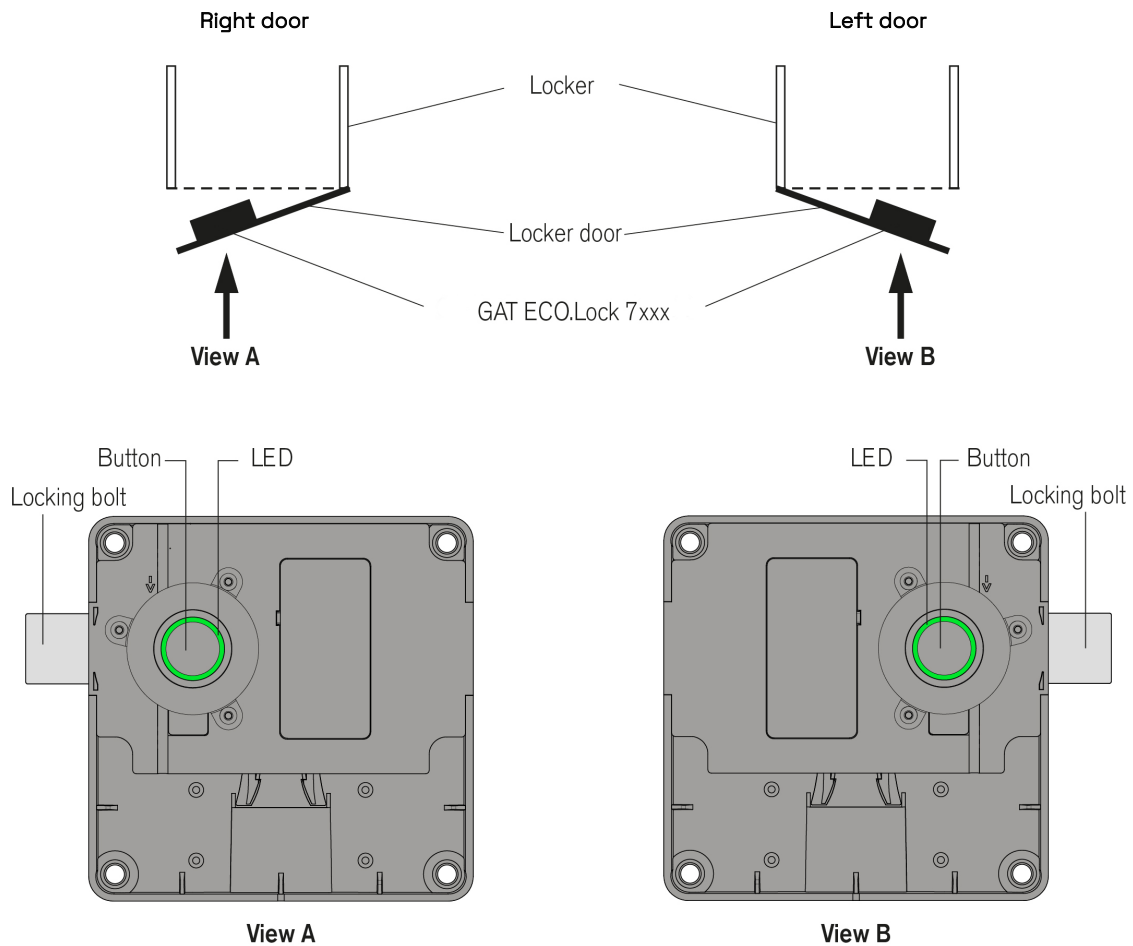
Fig. 3.1 – Locker door hinge definition (left / right)
