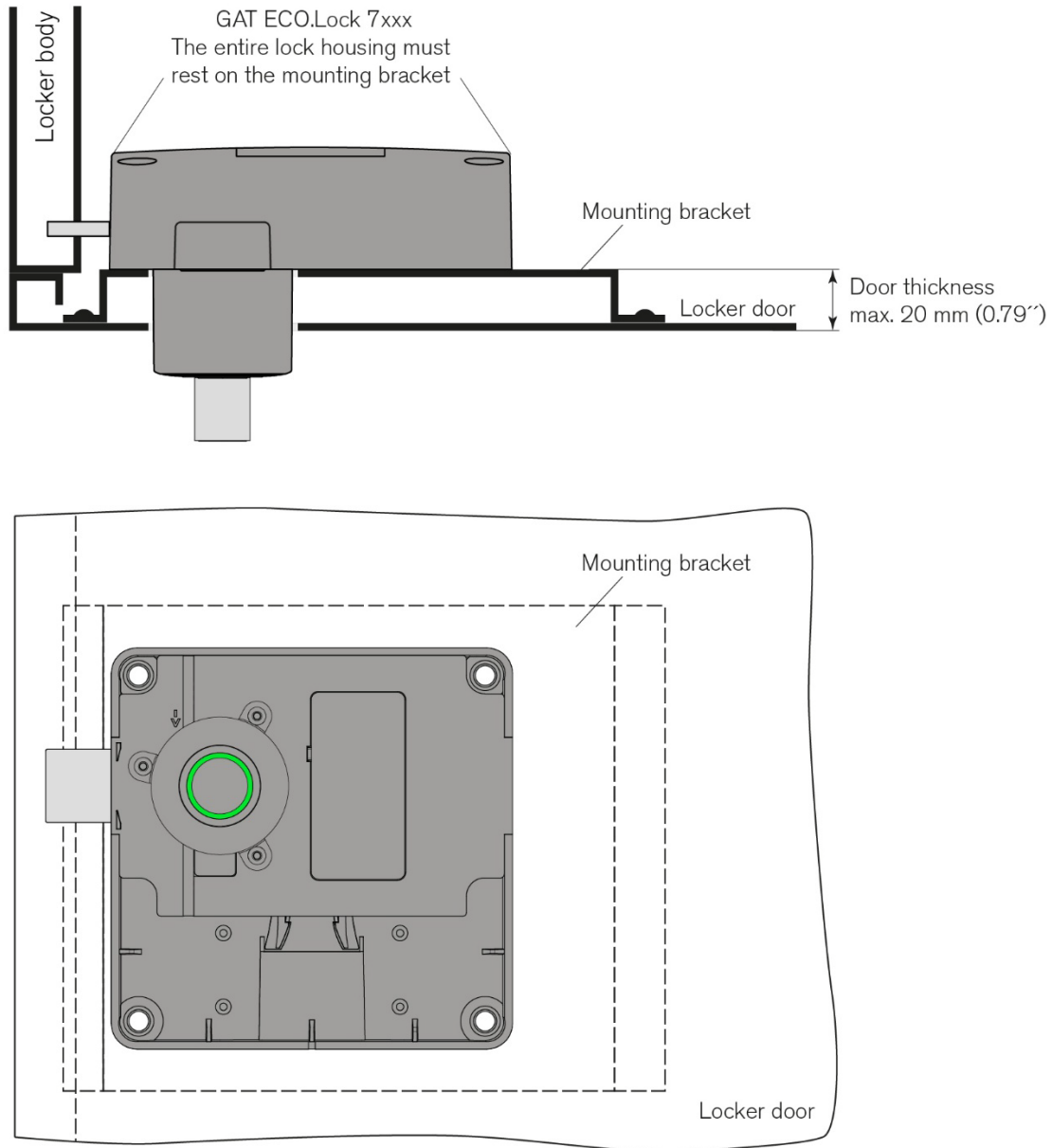
Fig. 3.10 – Installation of the GAT ECO.Lock on a single-wall metallic door
