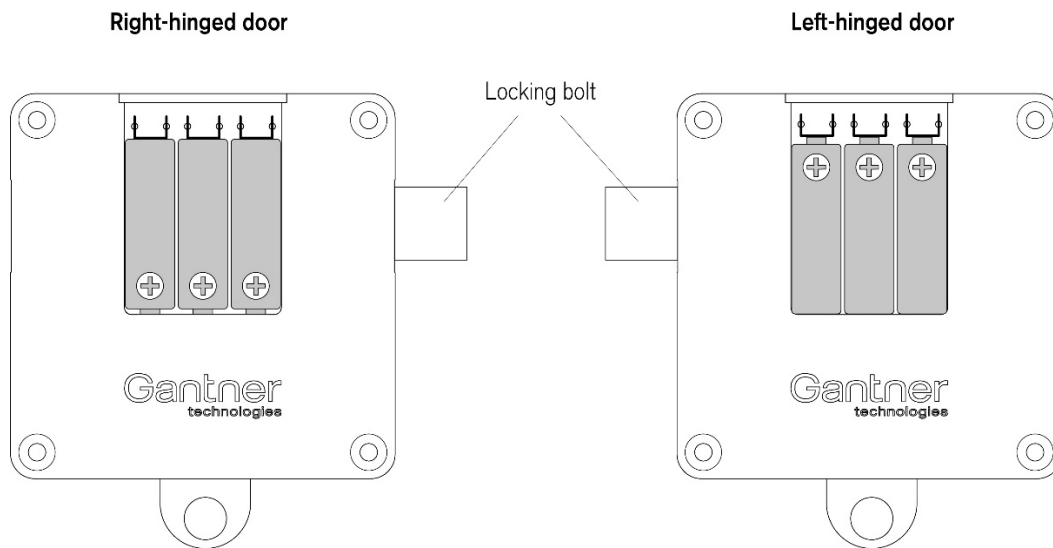
Fig. 4.2 – Correct battery polarity
