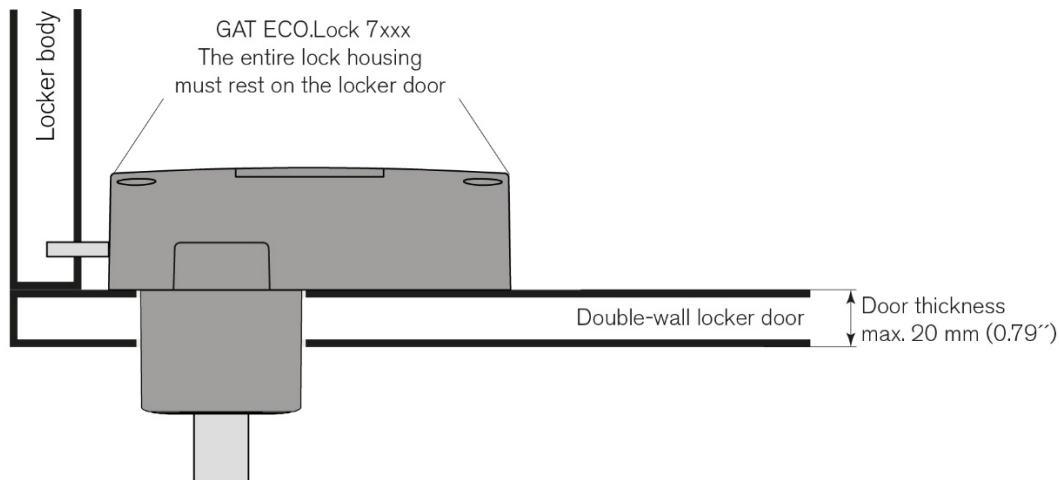
Fig. 3.11 – Installation of the GAT ECO.Lock on a double-wall metallic door
