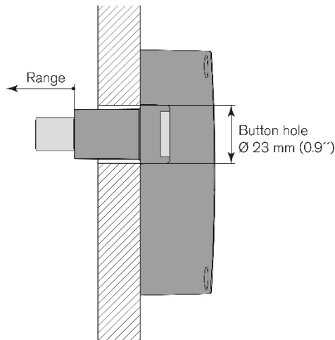
Fig. 3.4 – Diameter of the button drill hole for non-metallic doors
