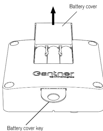
Fig. 4.1 – GAT ECO.Lock battery compartment
