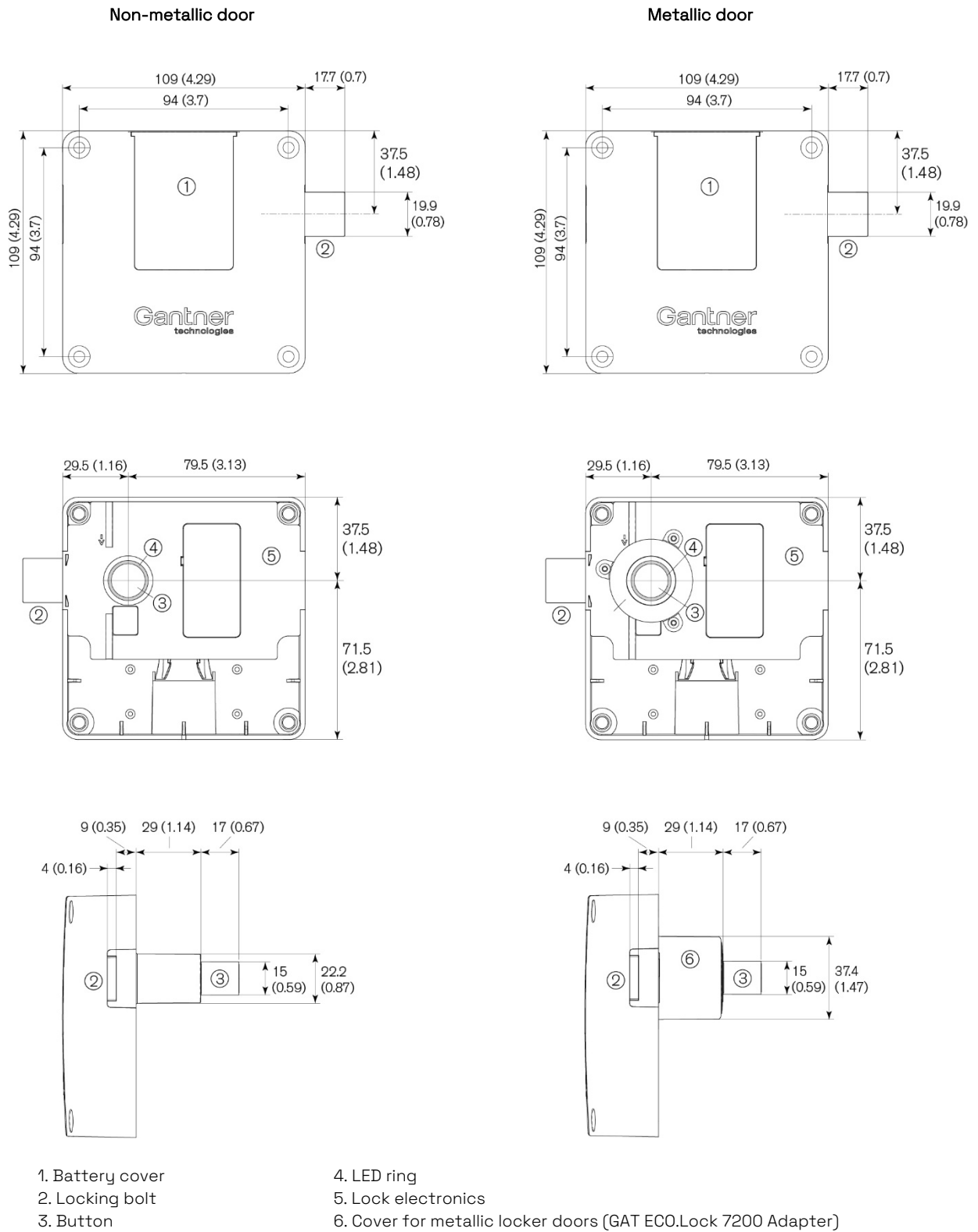
Fig. 3.3 – GAT ECO.Lock dimensions and components
